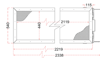
Air Discharge View
