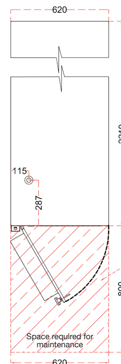
Top View
