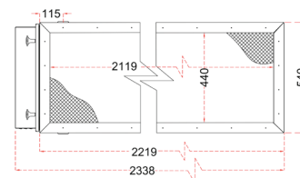
Air Intake View
